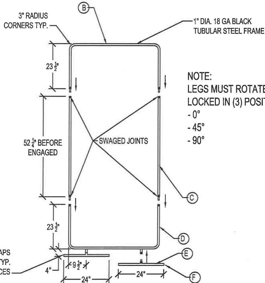
FRAME DISASSEMBLED (SNAP-LOCK FRAME ASSEMBLY)
